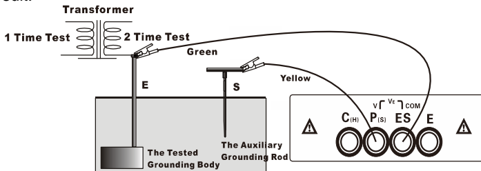
Commercial Grounding Body To Ground Voltage Test
